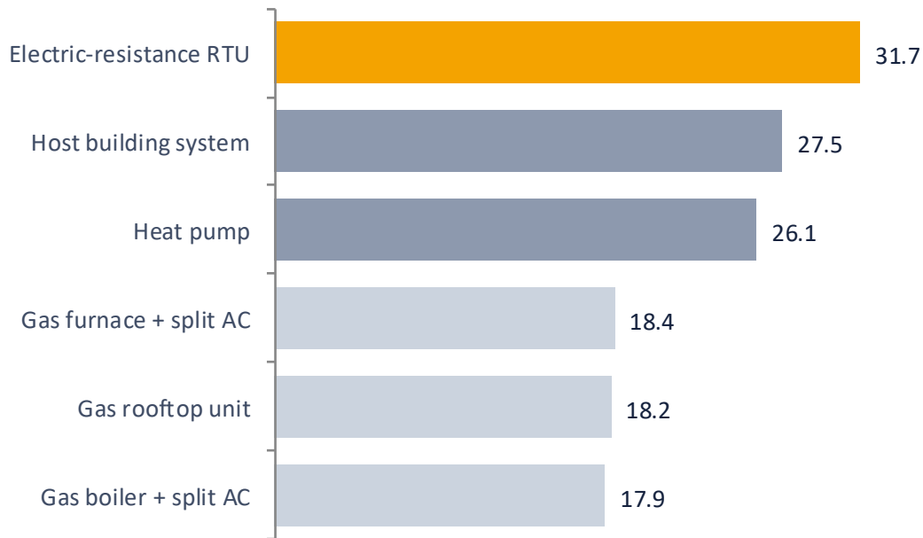
Median electricity intensity by HVAC type (kWh/sq ft/yr)
